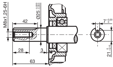
MOTORWELLE KW25x63 (S1)
