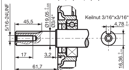
MOTORWELLE TP19x72 (V1)
