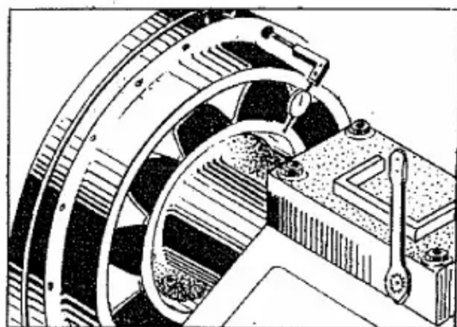
Fig.8 Correcting the Concentricity between Gearbox and Flywheel
