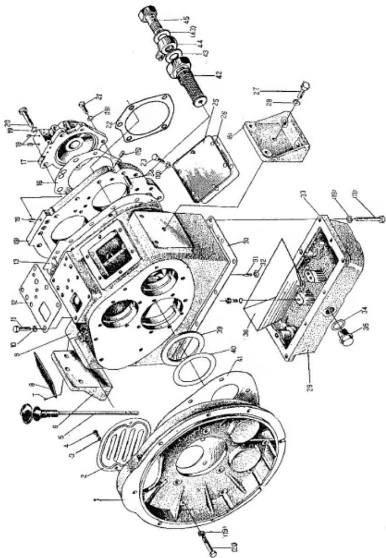
箱体部件 Housing Assembly
