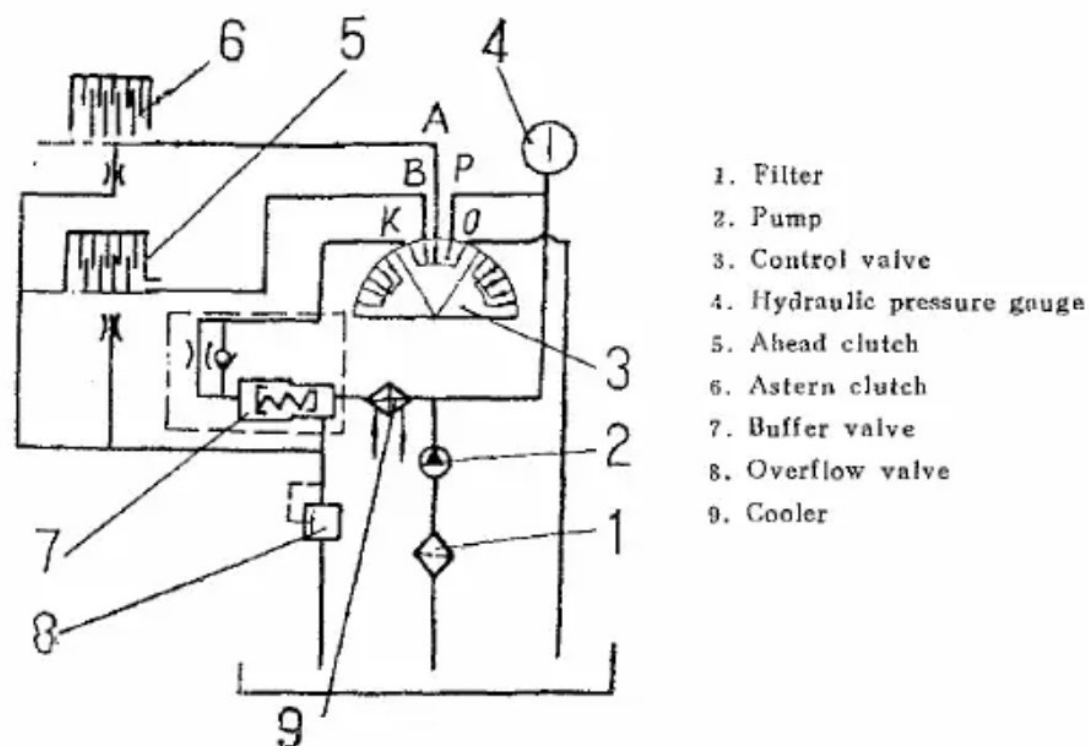
Fig.7 Diagram for Hydraulic System
