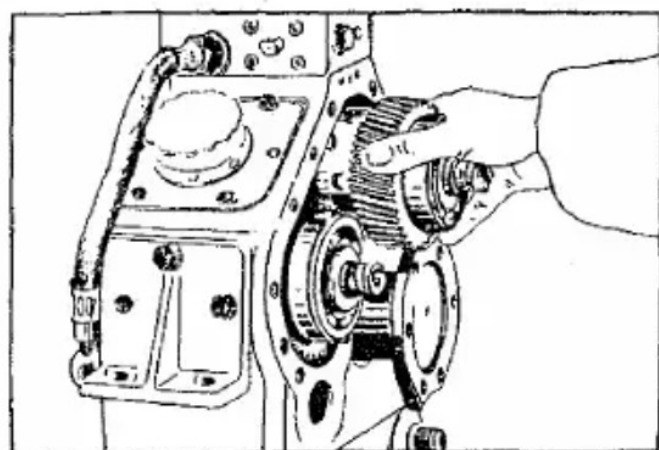
Fig.3 Dis- and Re-assembling of Clutch Assembly
