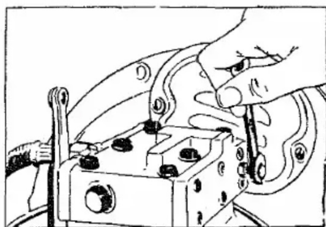
Fig.10 Adjusting of Initial Hydraulic Pressure
