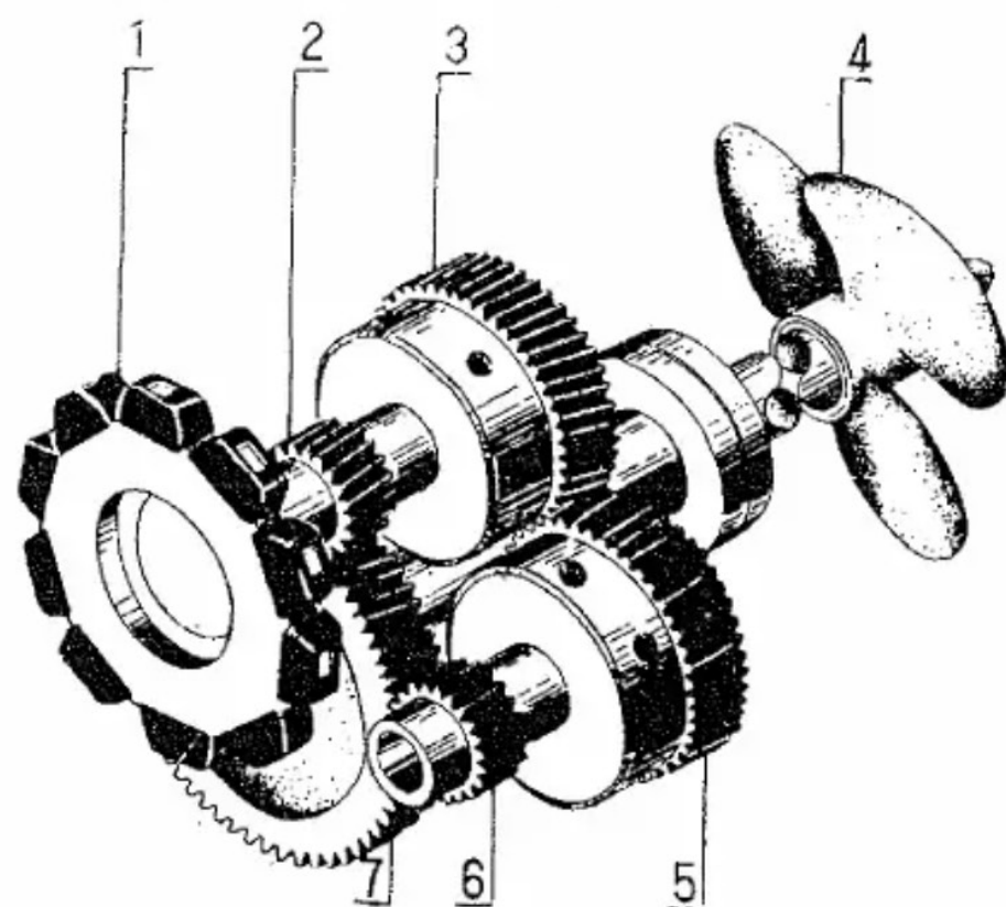
Fig.2 Diagram for Transmission System
