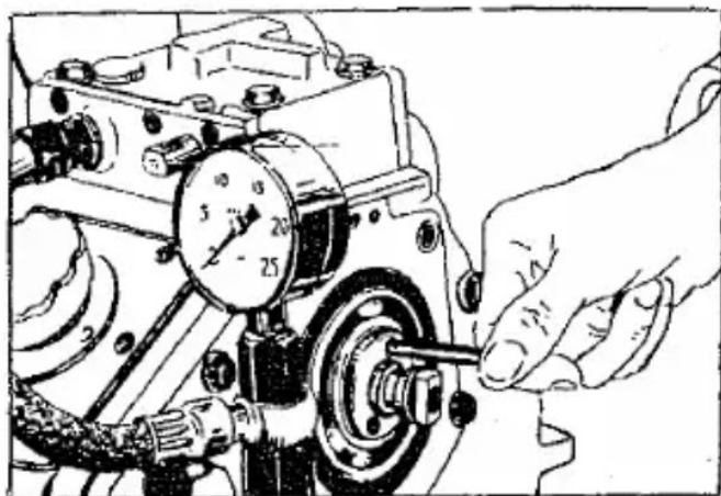
Fig.4 Using of the Emergency set
